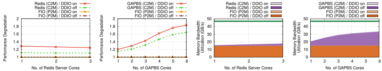
Figure 2: Enabling DDIO can worsen performance degradation for both C2M and P2M applications when the working set size does not fit in cache (left-right, a-d) (a, b) Performance degradation for C2M and P2M when they are colocated with DDIO on/off; (c, d) Memory bandwidth utilization when C2M and P2M are colocated with DDIO on/off.
